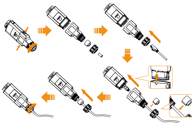
LAN mode (without water-proof ring)
