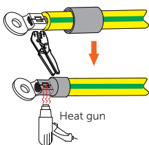
3 Crimp OT terminal and heat the heat-shrink tubing.
