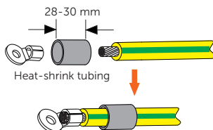
2 Insert the PE cable into the heat-shrink tubing and OT terminal.
