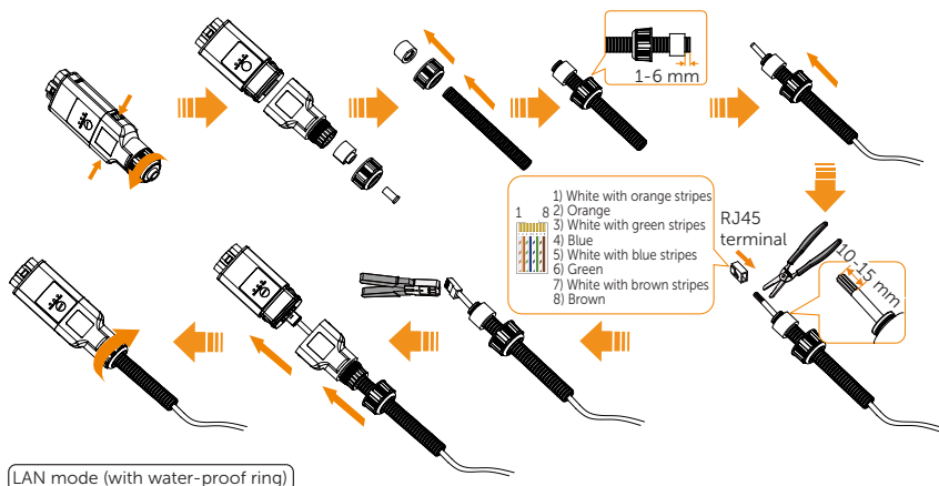
LAN mode (with water-proof ring)
