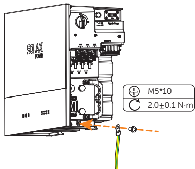
4 Connect the PE cable to the inverter and secure with the M5*10 screw.
