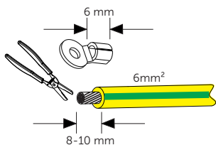
1 Strip the PE cable by wire stripper.
