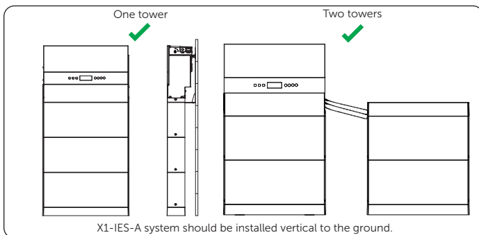
X1-IES-A system should be installed vertical to the ground.
