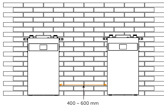
Option A: Floor Mounting
