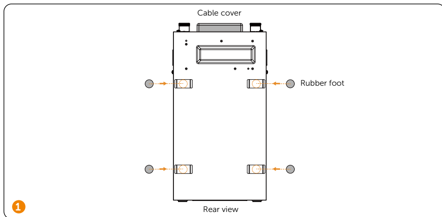
Installation of One Battery Pack (Stack Mounting)
