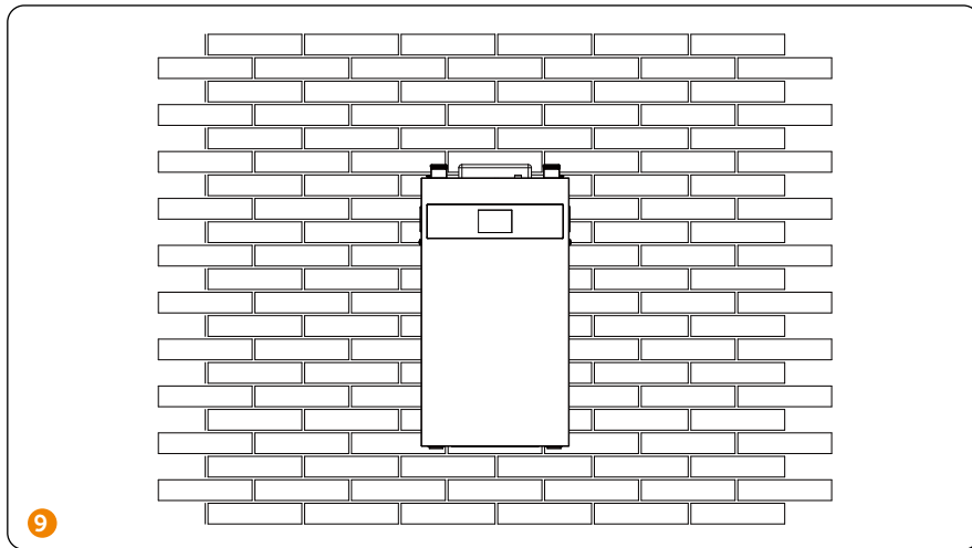
Installation of One Battery Pack (Stack Mounting)
