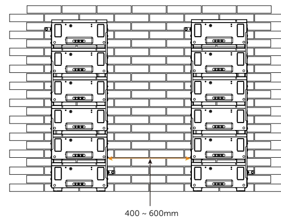
Option C: Stack Mounting
