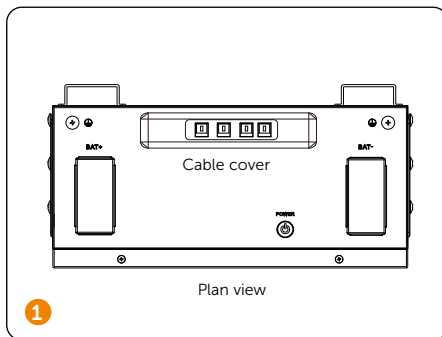
Installation of One Battery Pack (Wall Mounting)
