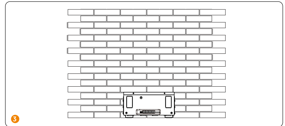
Two or More Battery Packs (Floor Mounting)
