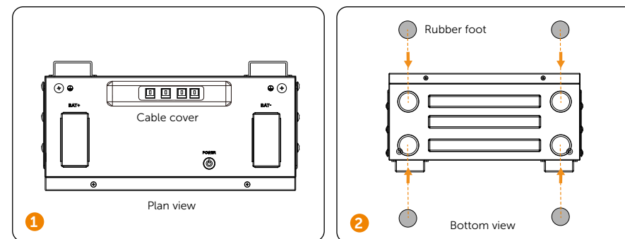
Installation of One Battery Pack (Floor Mounting)
