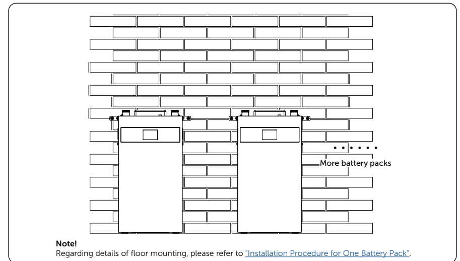
Two or More Battery Packs (Floor Mounting)
