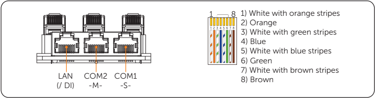
Figure 6-22 Communication ports
