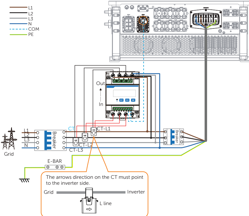
Wiring diagram of connecting a CT-connected meter
