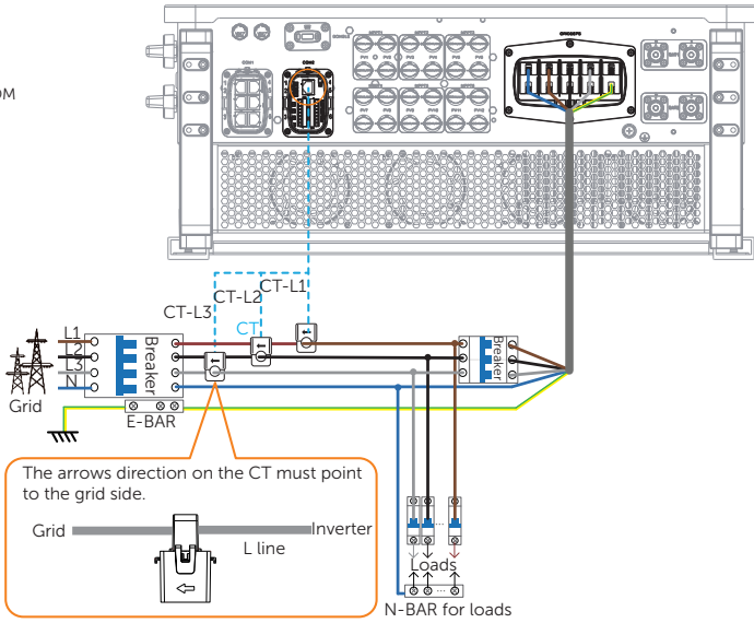
Wiring diagram of connecting a batch of CTs
